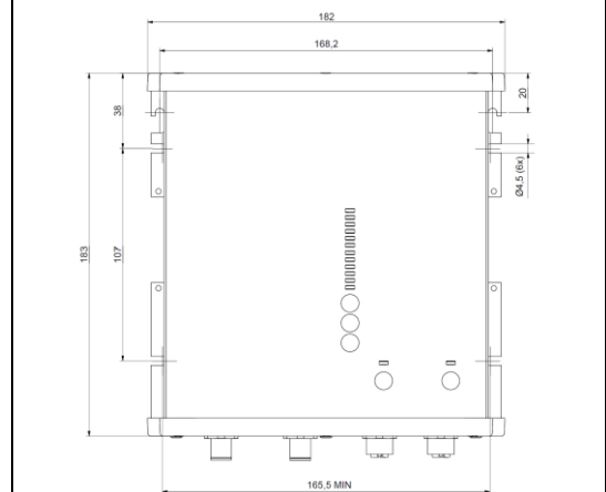
All dimensions in mm. Connectors X1 to X4 from left to right
